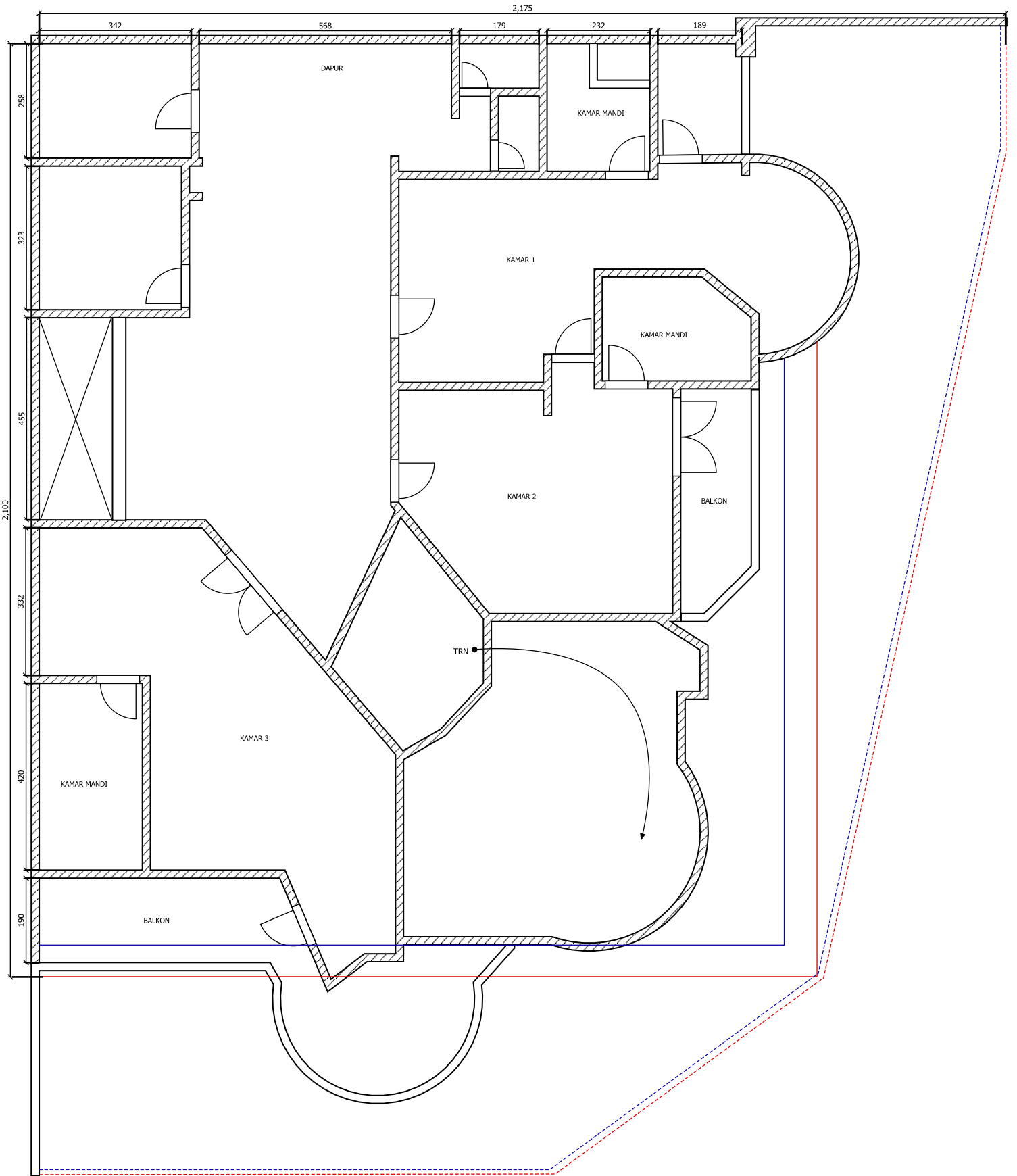
DENAH LANTAI 2
