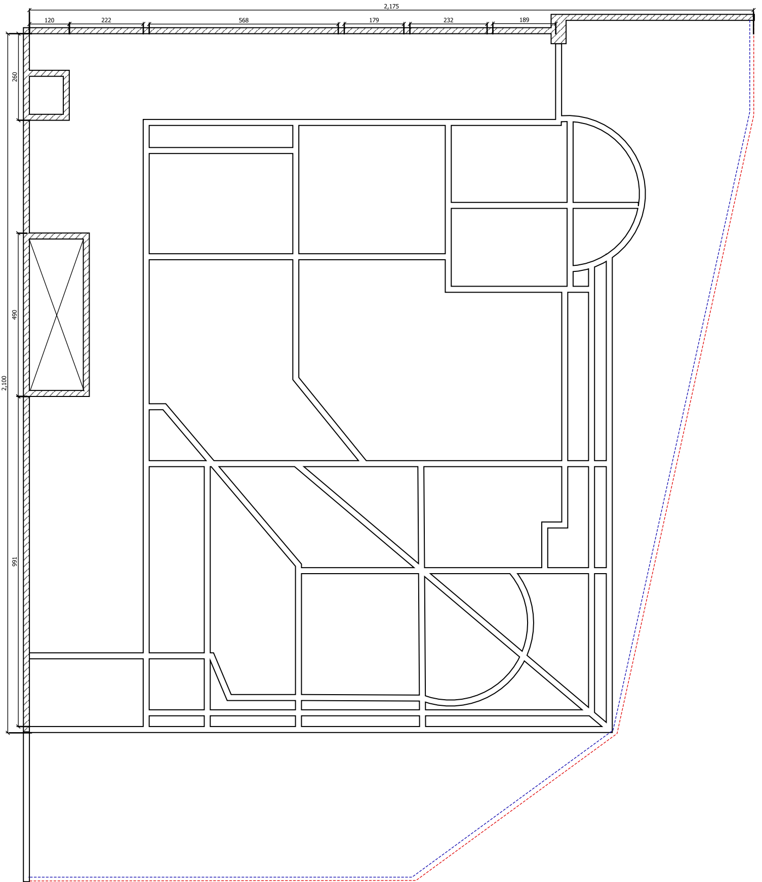
DENAH BALOK ATAP
