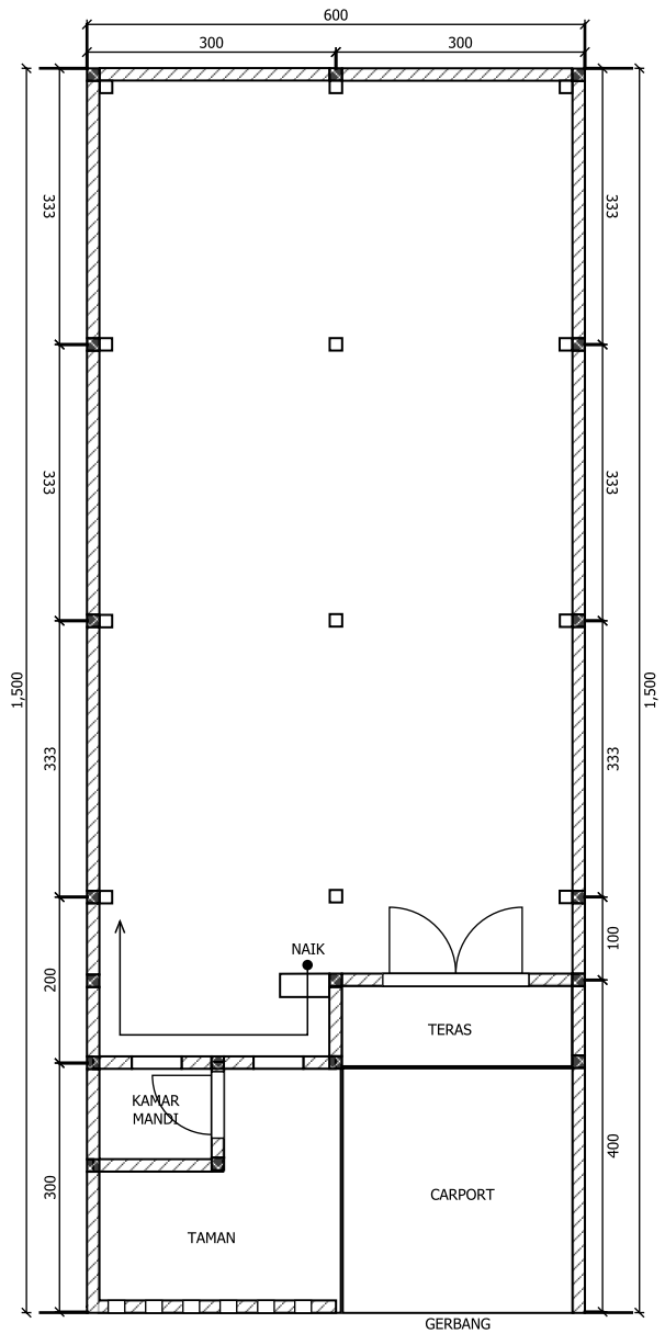
DENAH LANTAI 1 SKALA 1 : 100
