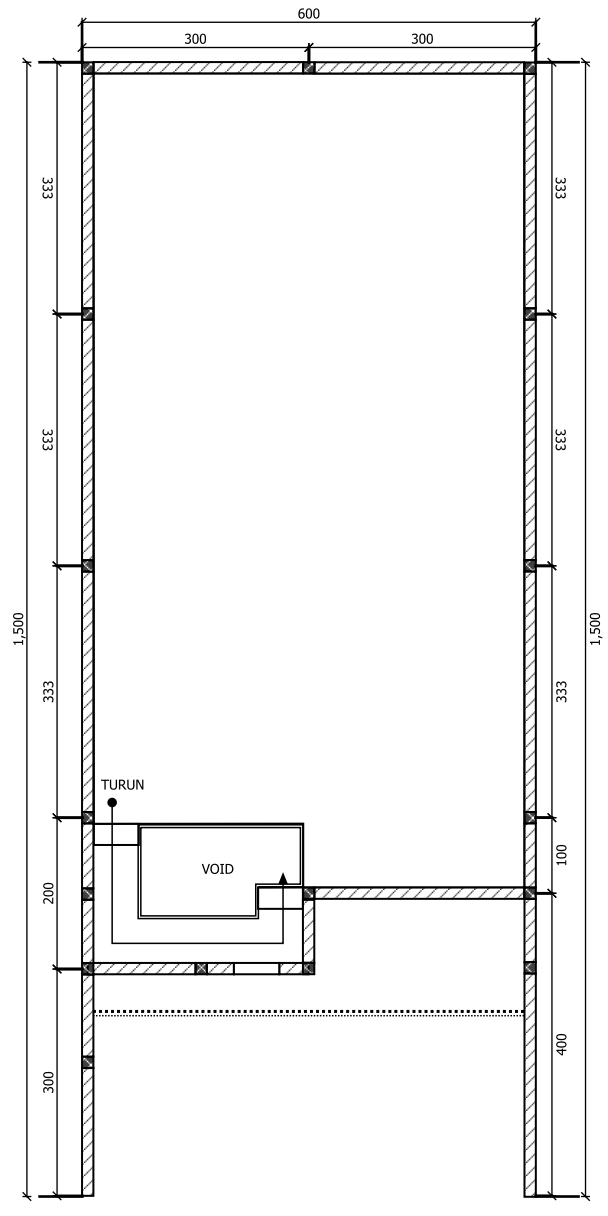
DENAH LANTAI 2 SKALA 1 : 100
