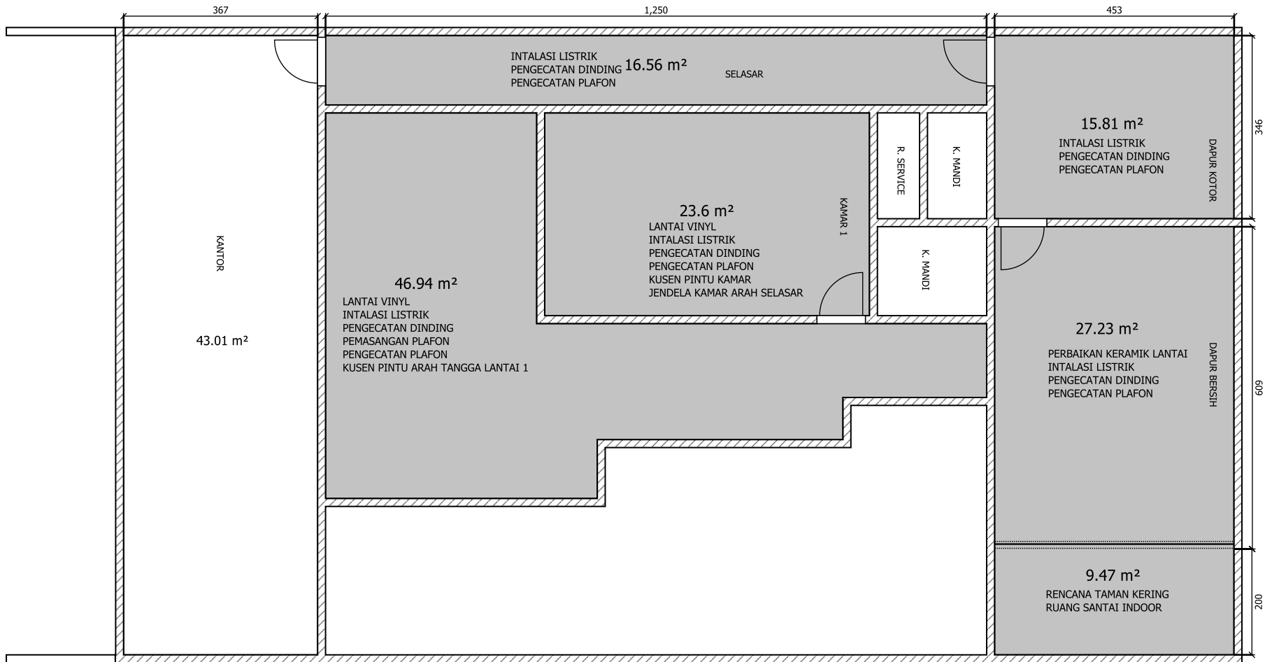
DENAH LANTAI 2 SKALA 1 : 100
