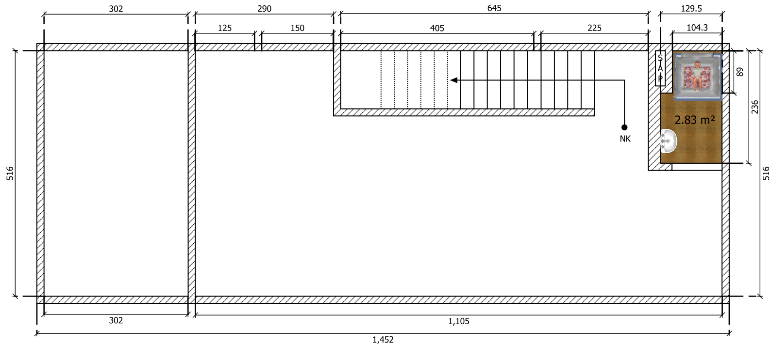
DENAH LANTAI 3 SKALA 1 : 75
