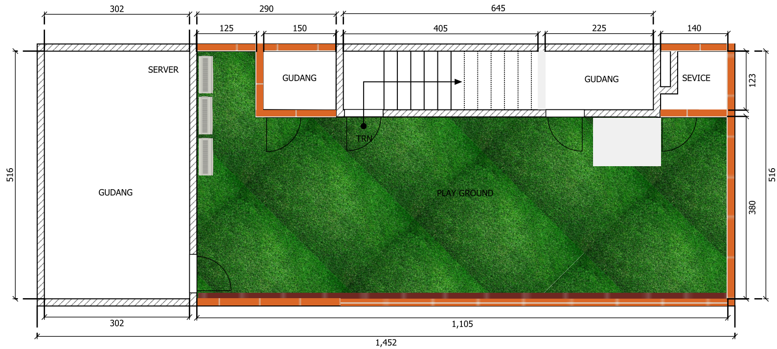
DENAH LANTAI 4 SKALA 1 : 75
