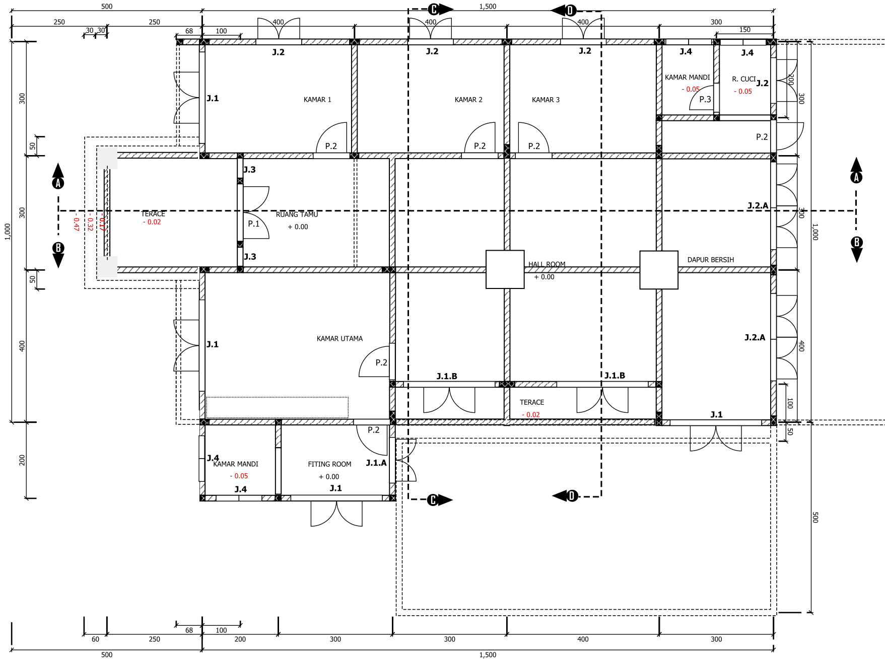
DENAH KUSEN LANTAI 1 SKALA 1 : 100
