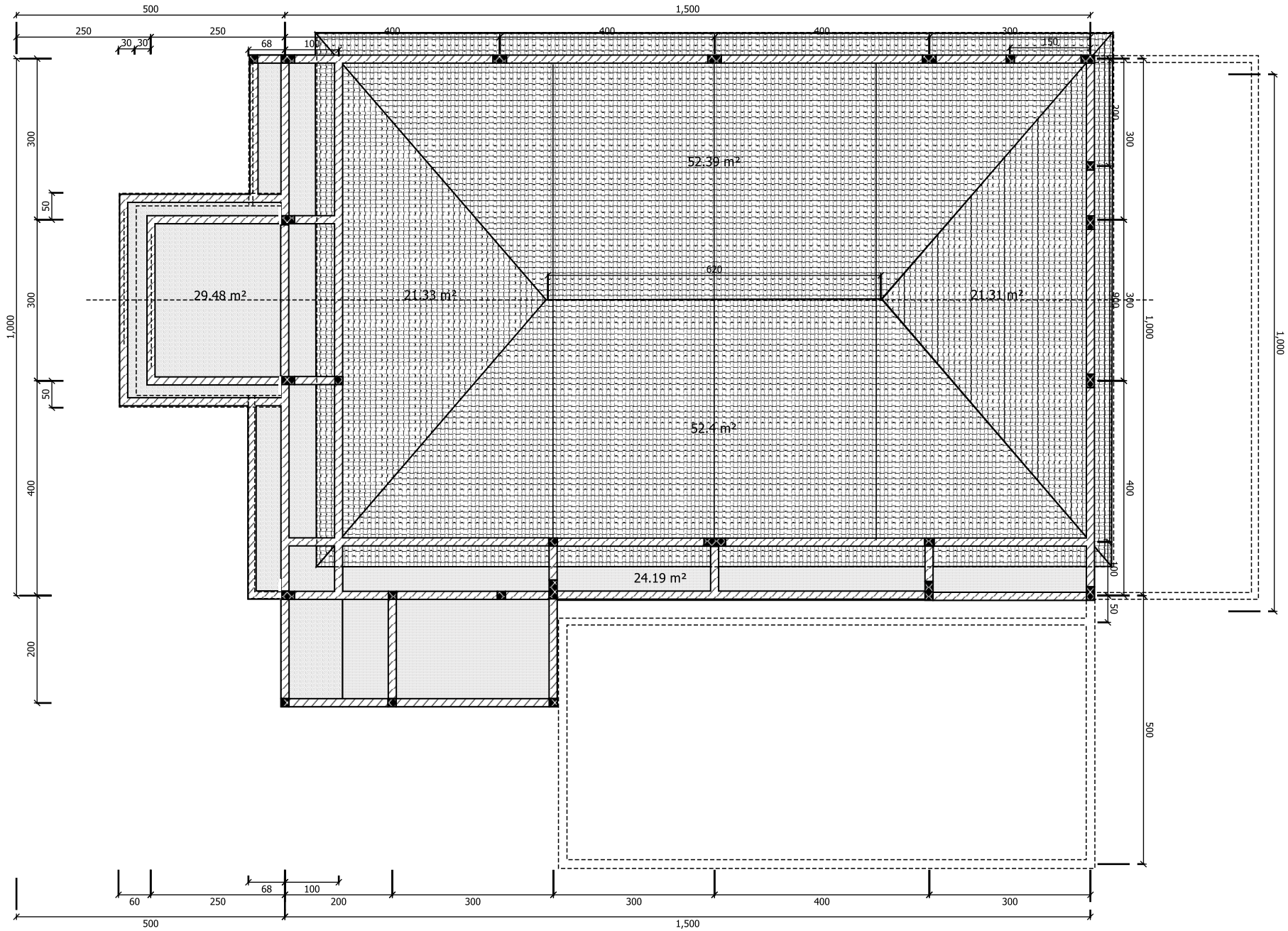
DENAH ATAP SKALA 1 : 100
