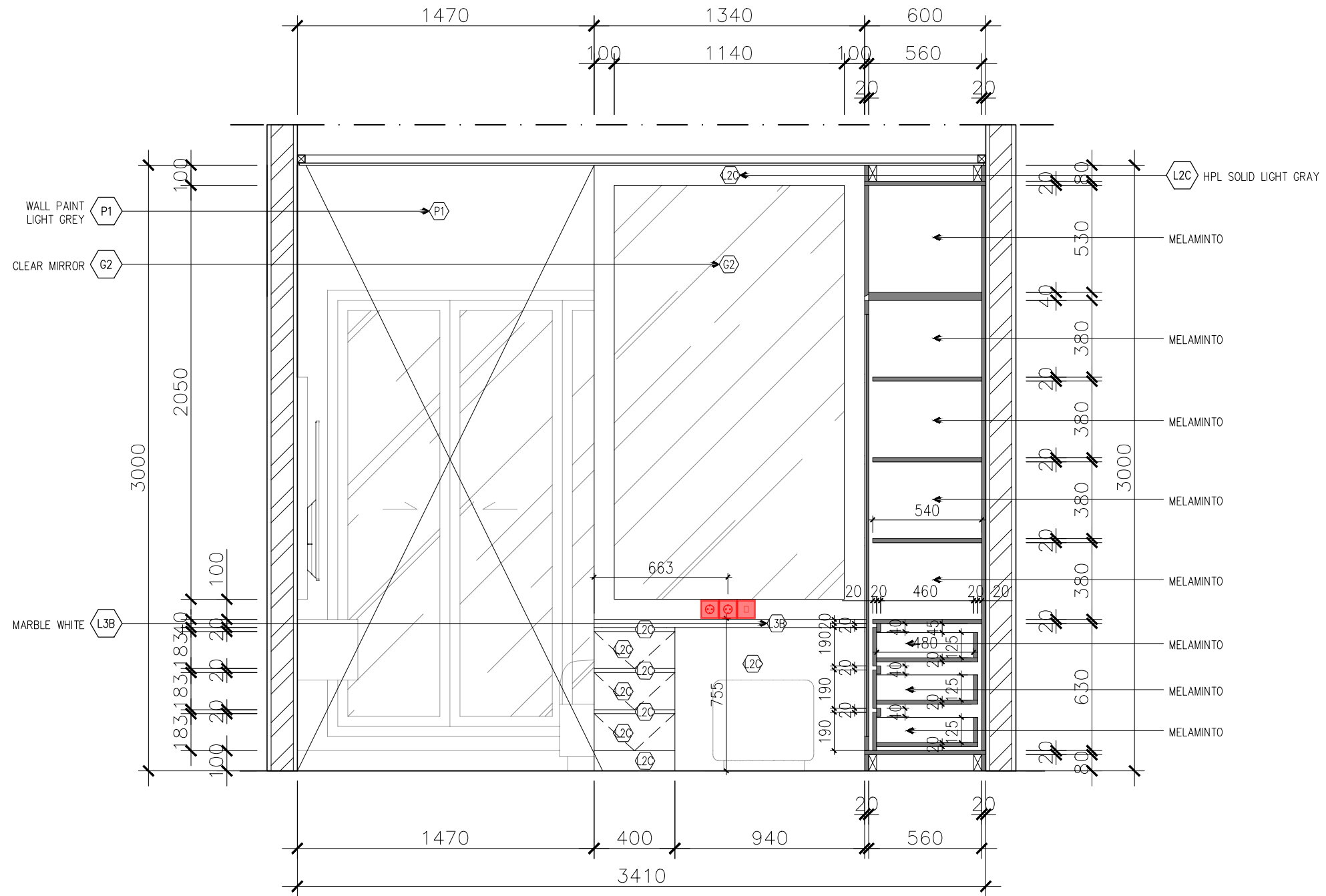
Section 2 Scale 1:25
