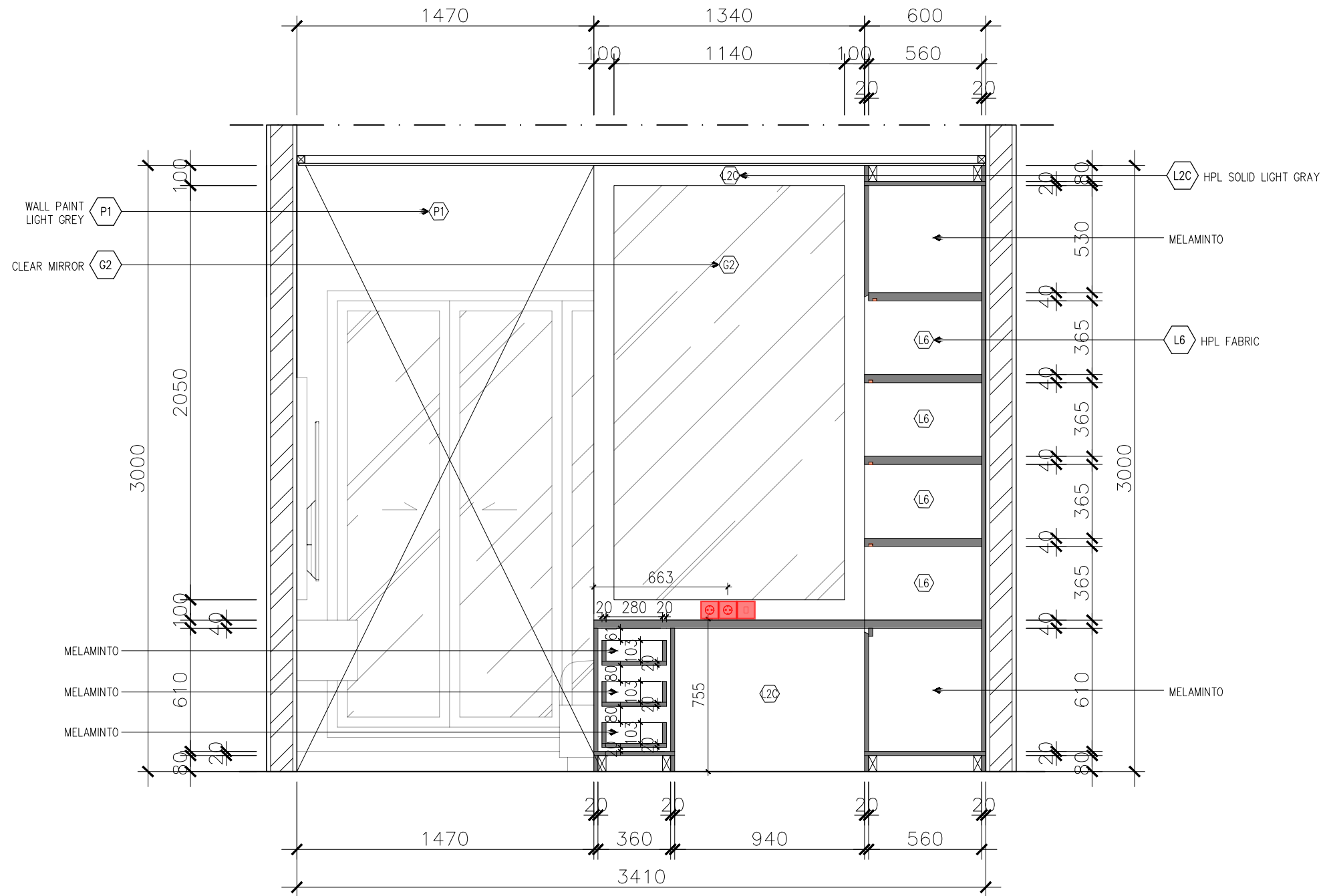
Section 1 Scale 1:25
