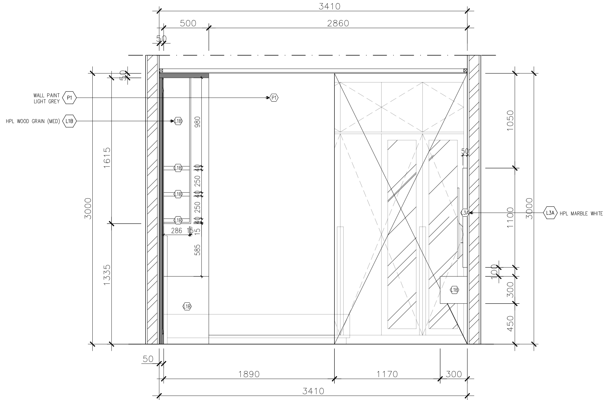
Section 1 Scale 1:25
