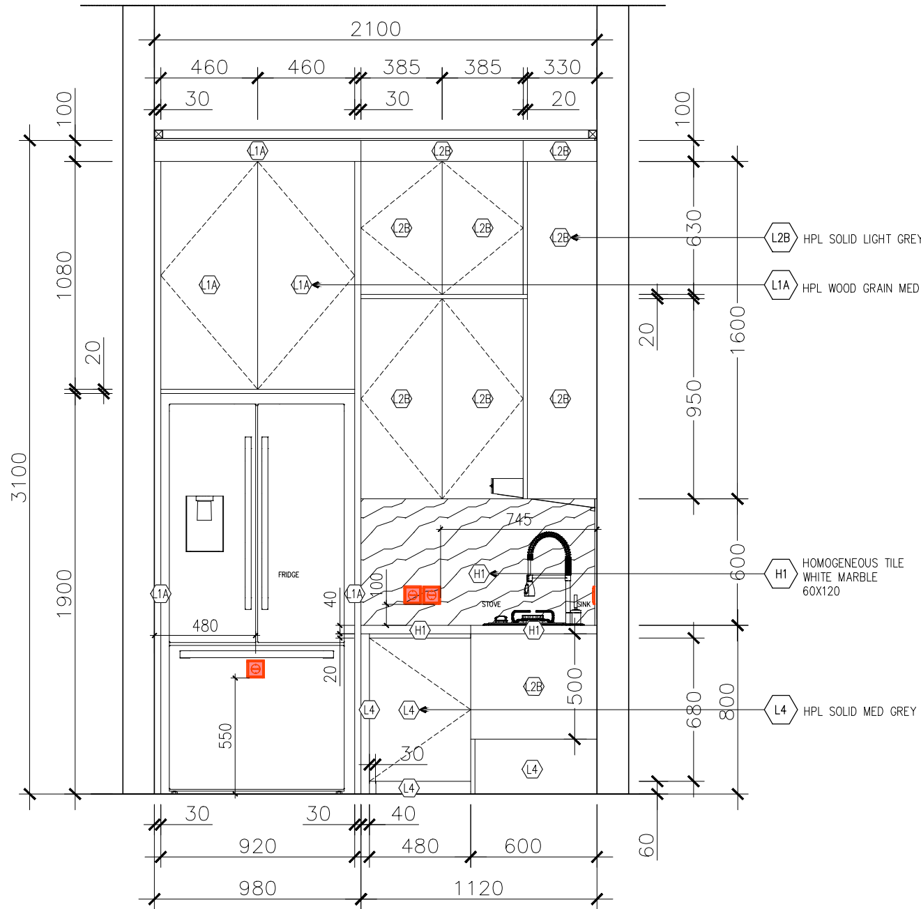
ELEVATION A KITCHEN SCALE 1:25
