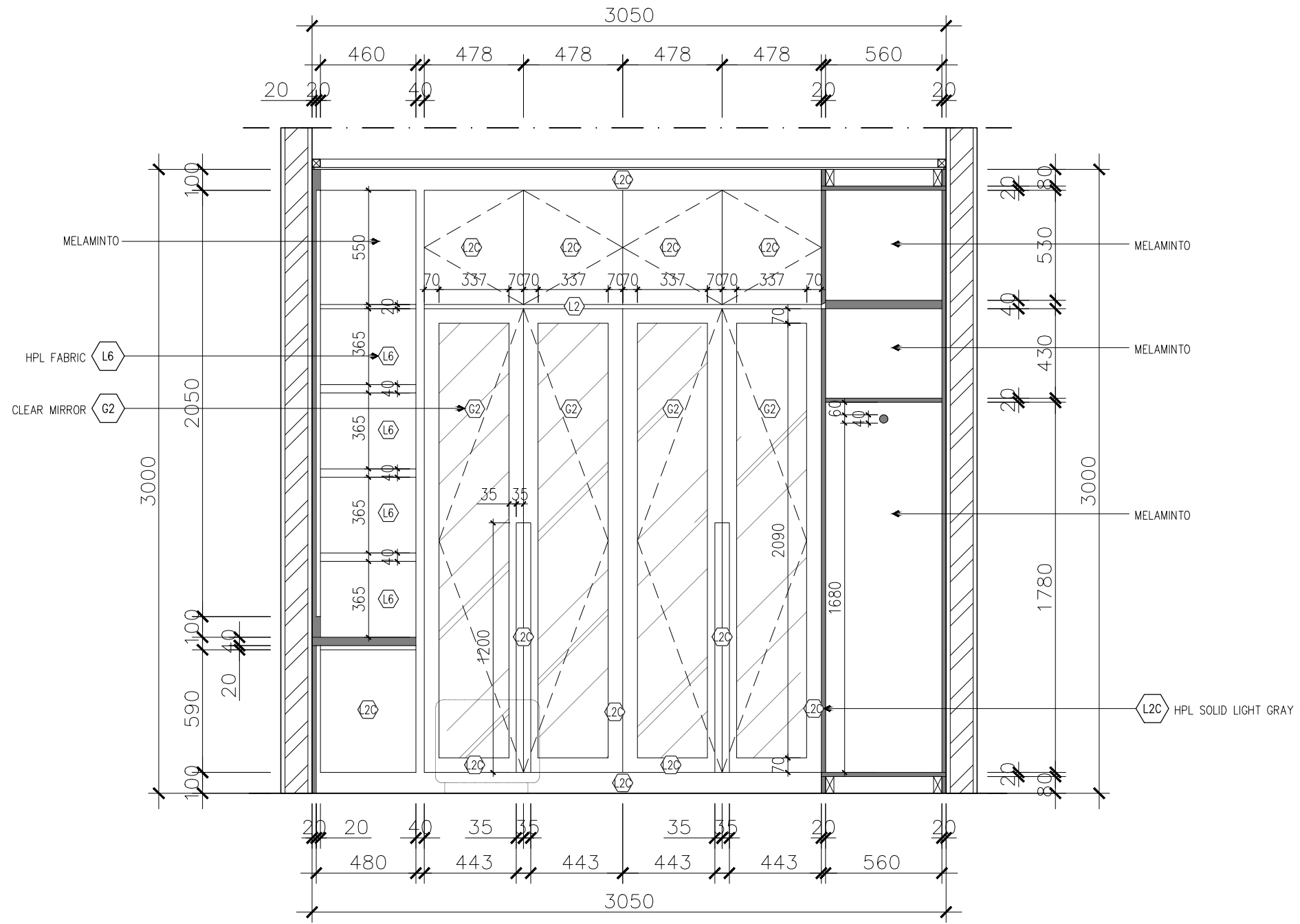
Section 6 Scale 1:25
