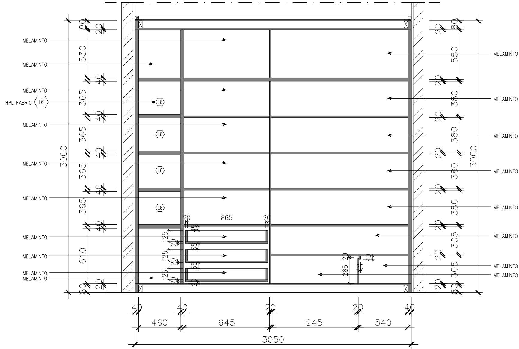
Section 5 Scale 1:25
