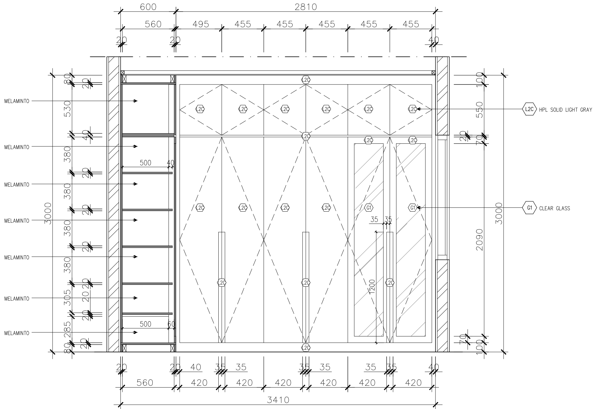
Section 3 Scale 1:25
