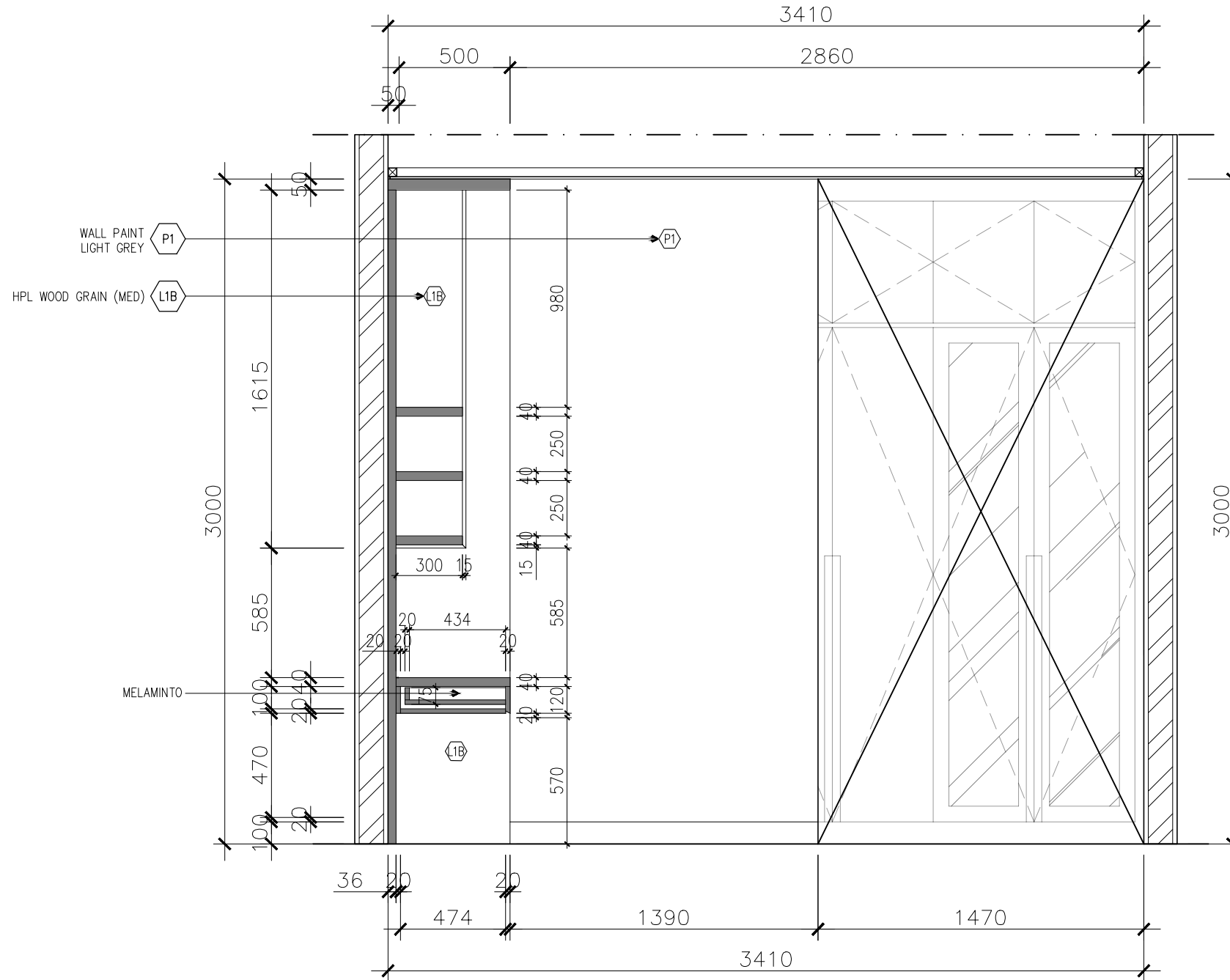
Section 5 Scale 1:25
