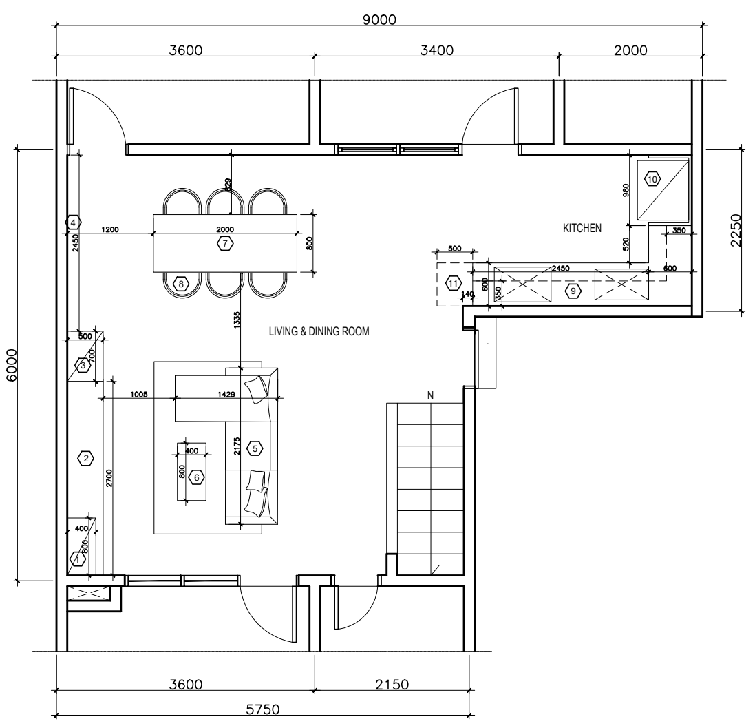
Layout Lt.1 Scale 1:75
