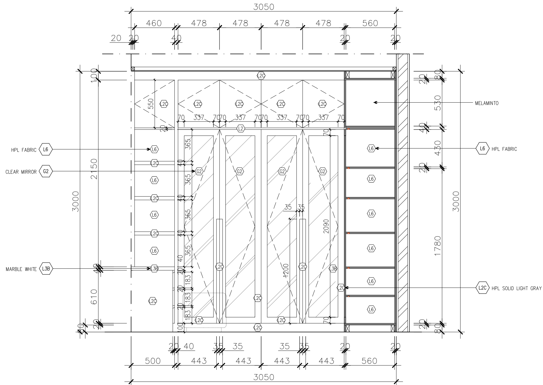
Section 8 Scale 1:25
