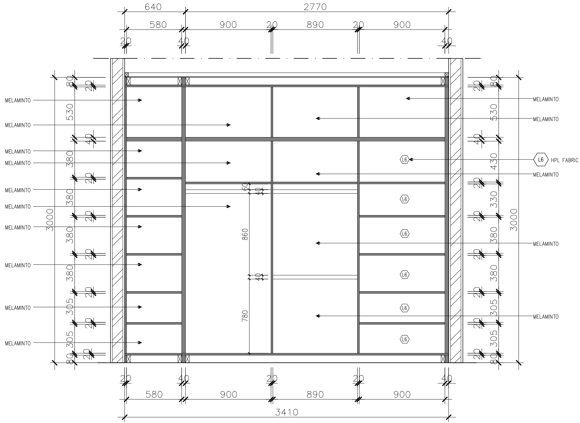
Section 4 Scale 1:25
