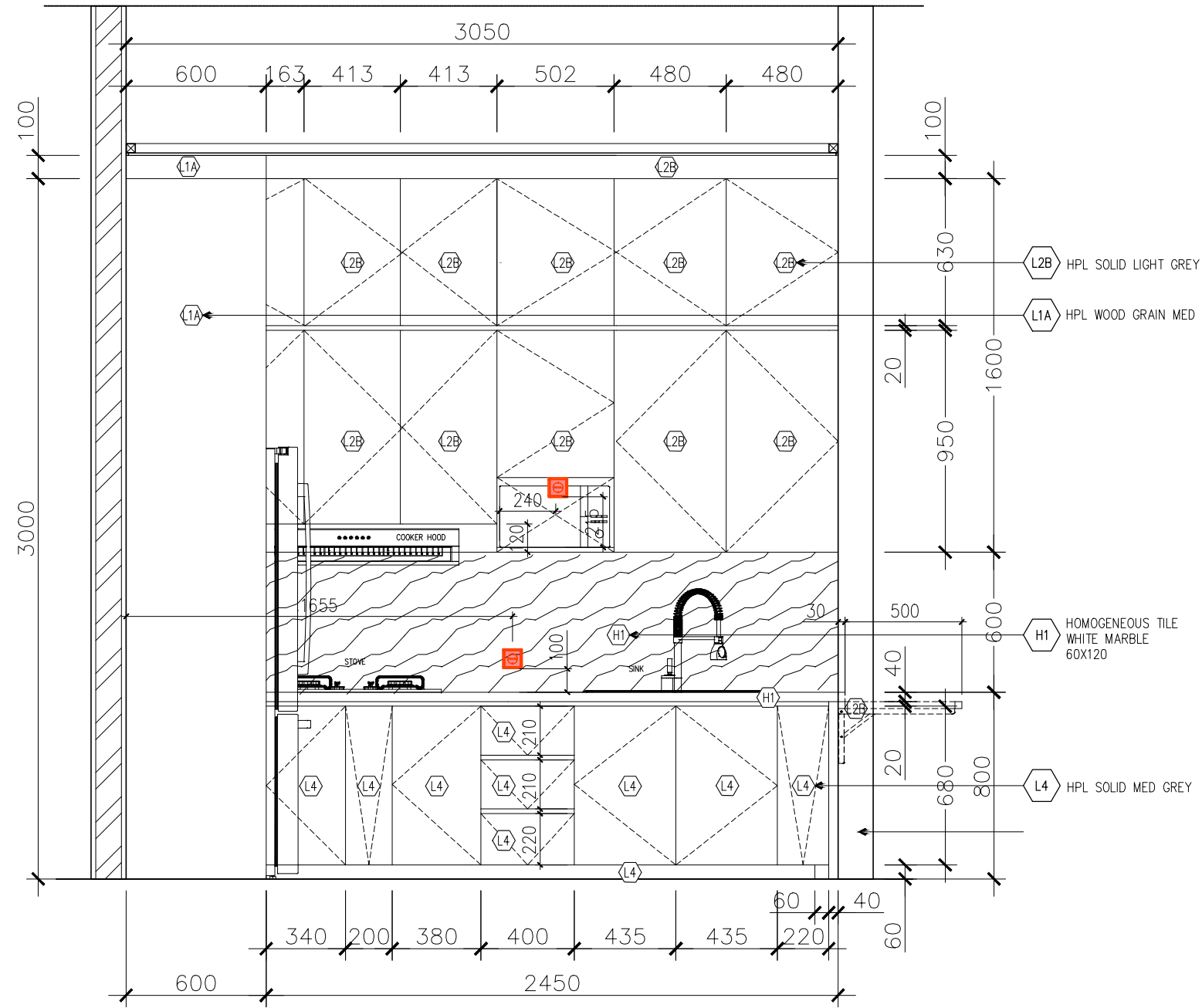
ELEVATION B KITCHEN SCALE 1:25
