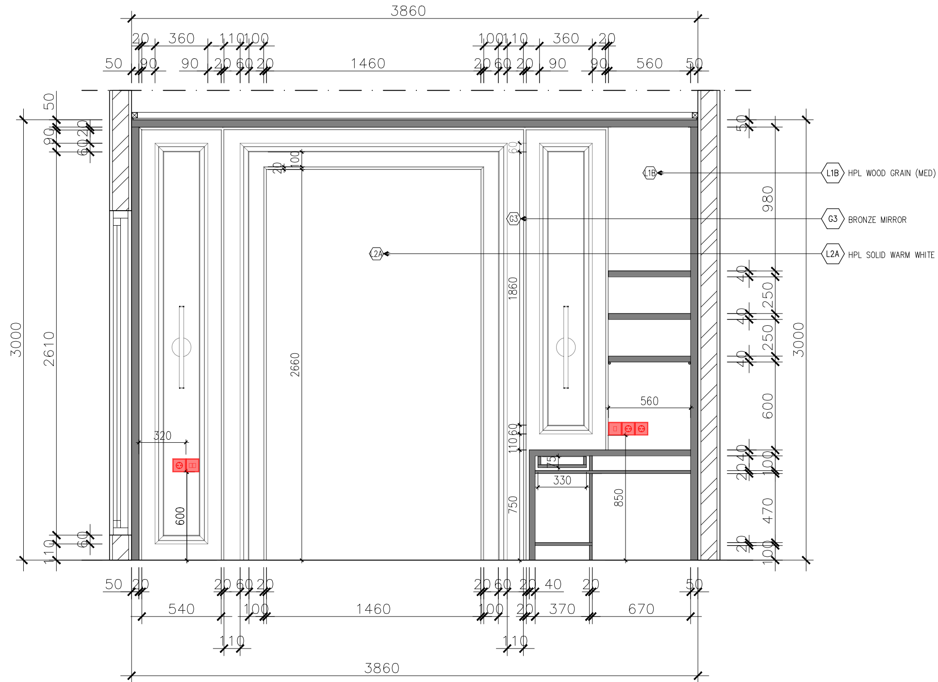
Section 6 Scale 1:25
