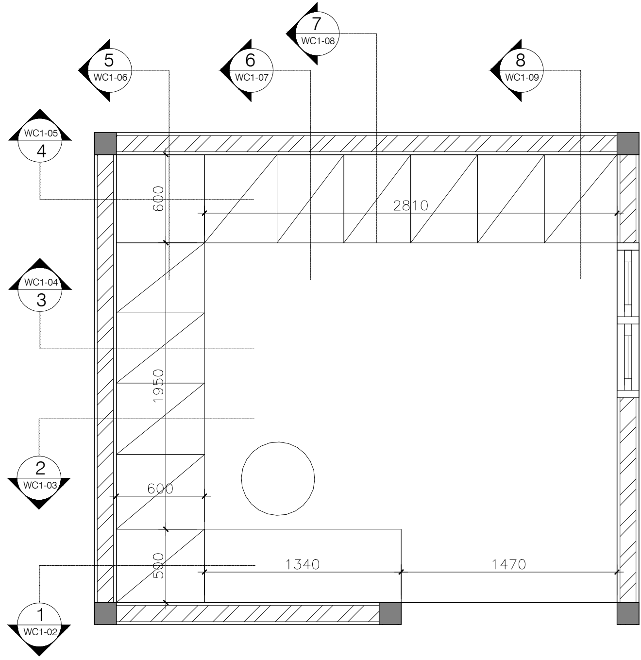
Layout Walk in Closet Scale 1:25
