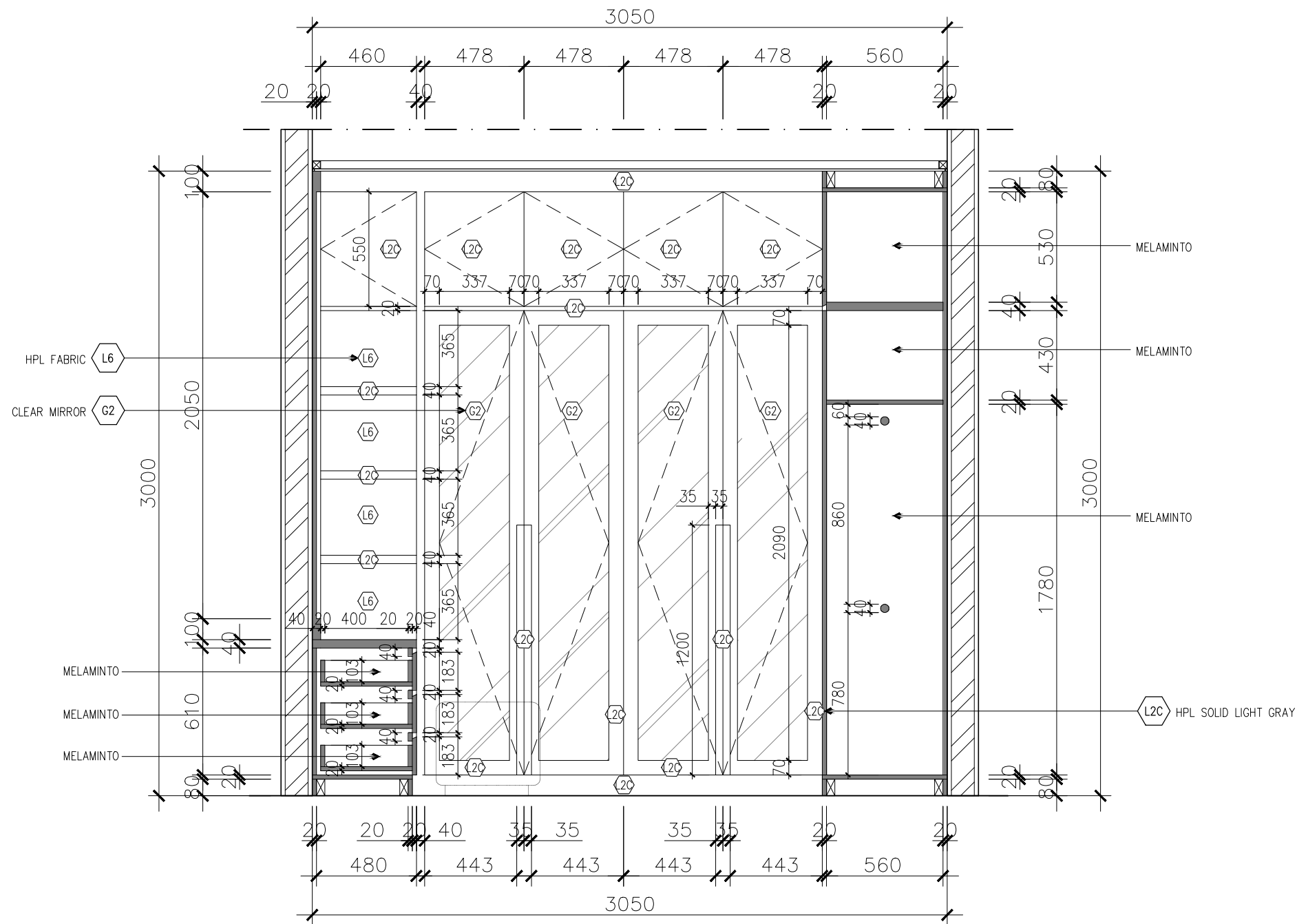
Section 7 Scale 1:25
